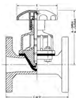
Flanged DN15 – DN50
