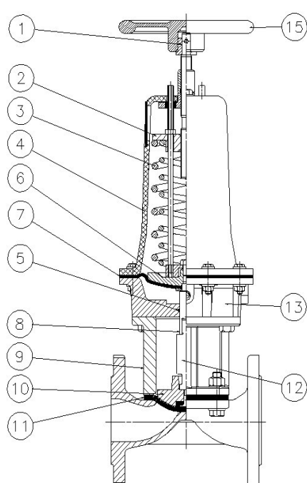
Spring Close
