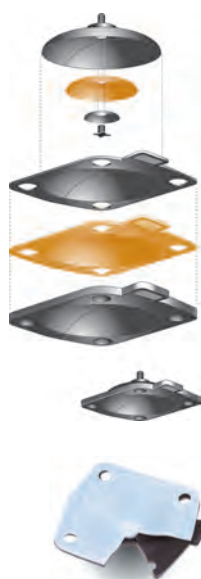
PTFE Diaphragm
