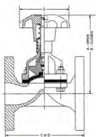
Flanged DN15-DN50
