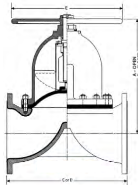
Flanged DN200-DN350
